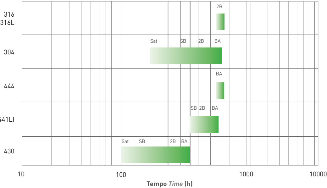
Resistenza in camera a nebbia salina in funzione della finitura superficiale (test eseguito secondo standard ASTM B117). Resistance in salt spray fog chamber test based on the surface finish (test performed according to ASTM B117 standard).
