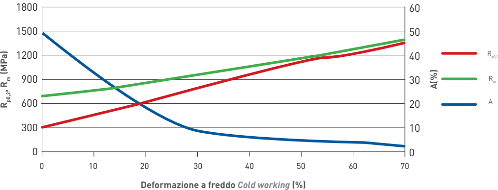
CURVA INCRUDIMENTO WORK HARDENING CURVE
