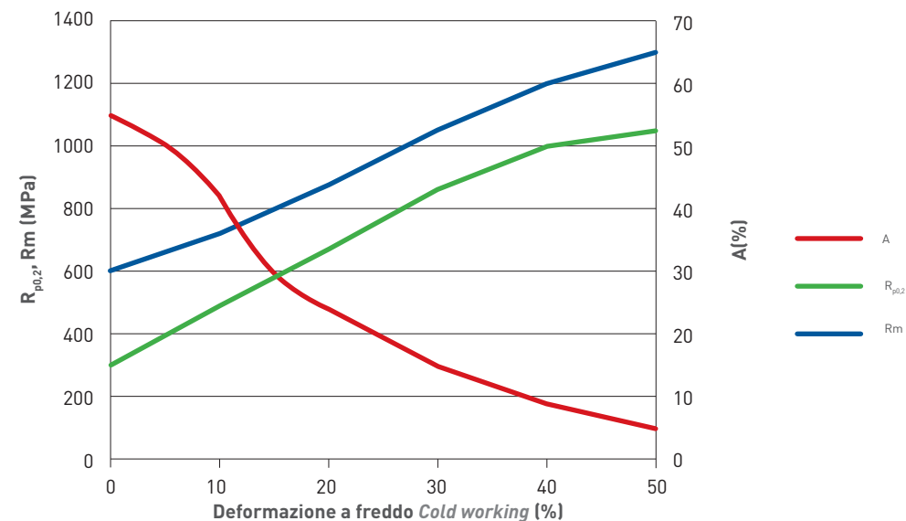
CURVA INCRUDIMENTO WORK HARDENING CURVE
