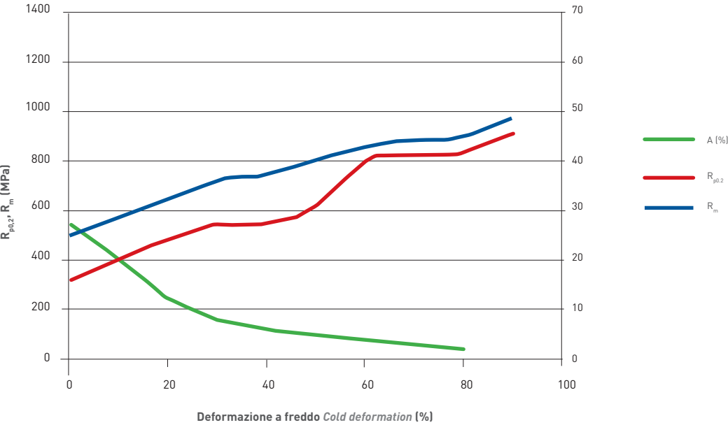
CURVA INCRUDIMENTO WORK HARDENING CURVE
