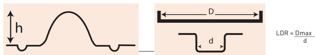
Schema del calcolo dell'indice Erichsen e del LDR (test Swift). Calculation diagram of the Erichsen index and LDR (Swift test).
